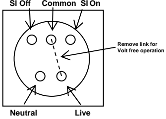
TLX RFP(V) receiver
