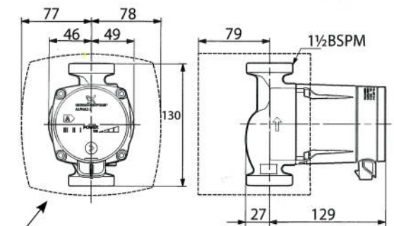
OPTIONAL INSULATION SHELL Part No:505821
